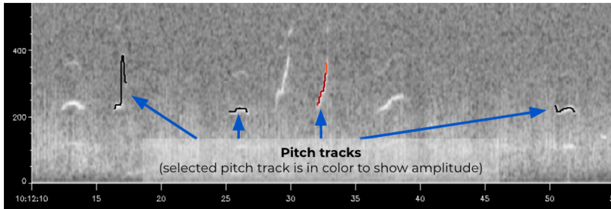
Image 2: Spectrogram showing the pitch tracks (black and color lines) tracing the humpback whale vocalizations. As the analyst clicks between pitch tracks, the LFDCS will highlight the selected pitch track in color showing the amplitude of that sound (warmer colors are louder, cooler colors are quieter). Surrounding pitch tracks will appear black until the analyst clicks to the left or right to select a different pitch track. The LFDCS will automatically center the selected pitch track in the spectrogram window.
